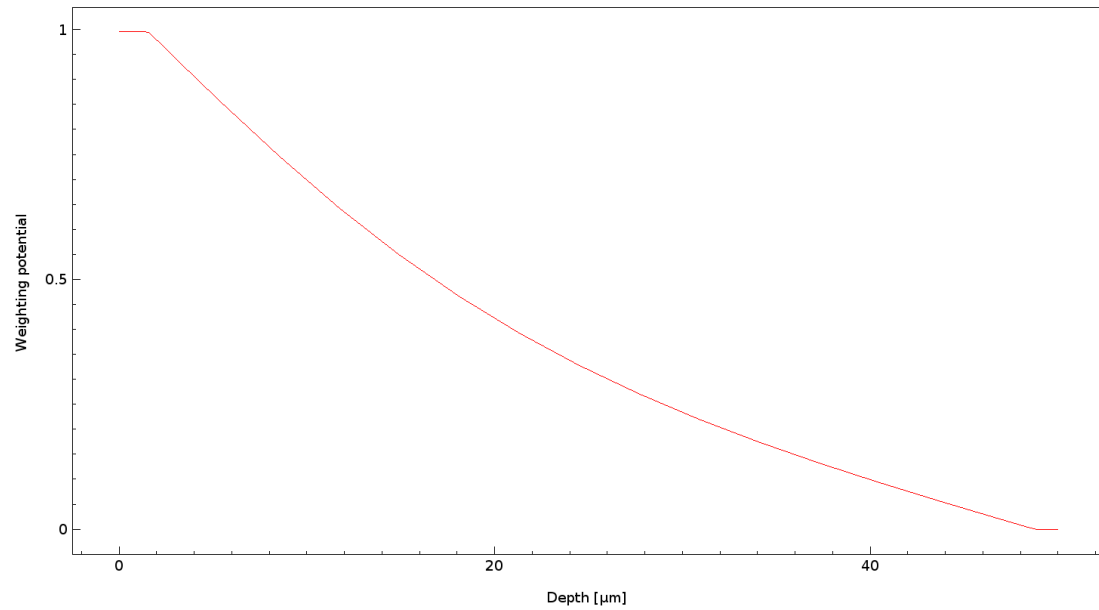
Weighting potential at pixel centre
