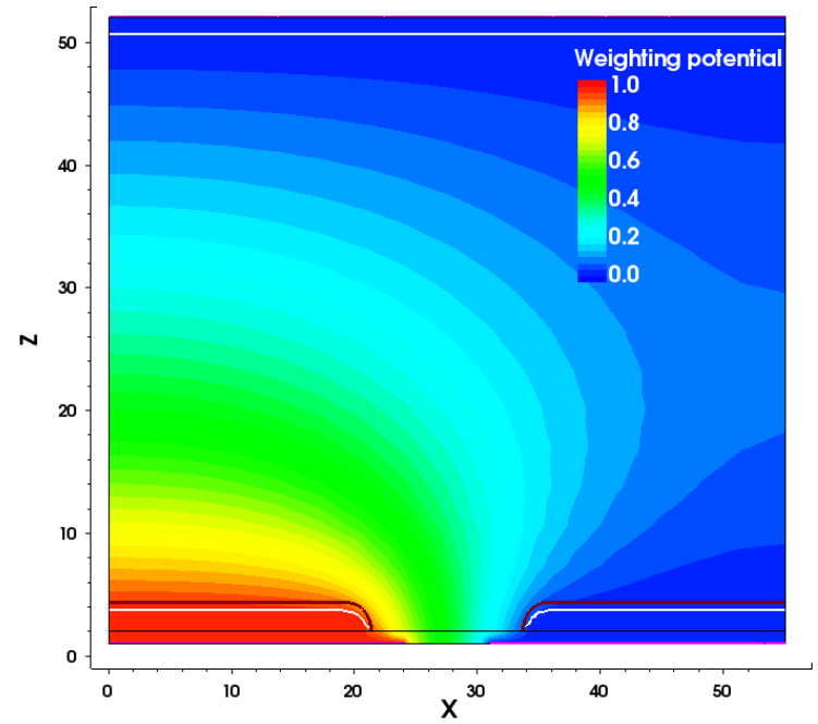
Weighting potential at pixel centre
