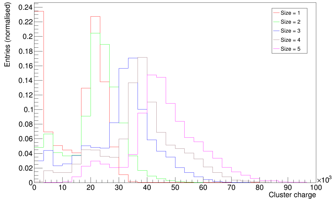
Charge for several cluster sizes (normalised)
