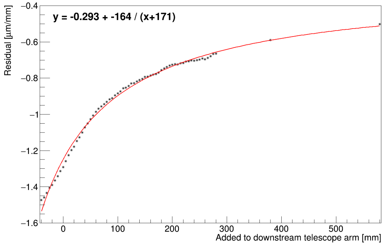
Effect of misaligned telescope
