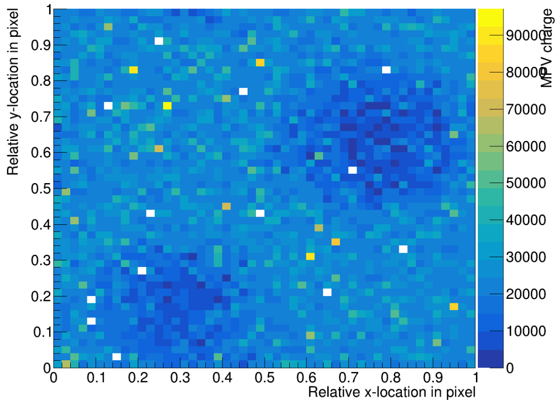
Charge map (Run 31618, 285 \mu\text{m} 3D, Vbias 40V, 0 degrees)
