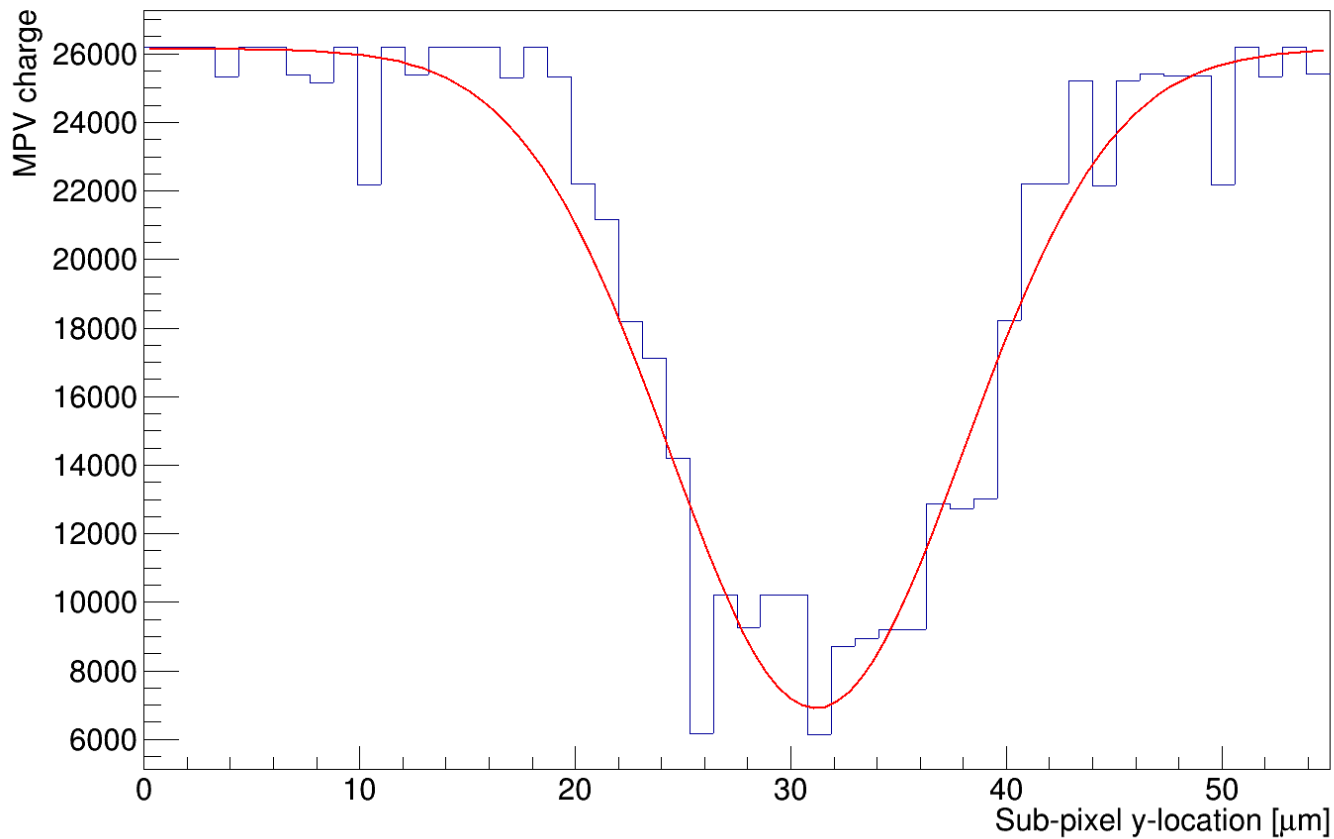
Charge distribution for middle column, part 9
