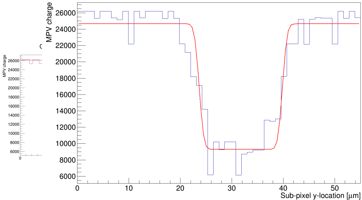
Charge distribution for middle column, part 9
